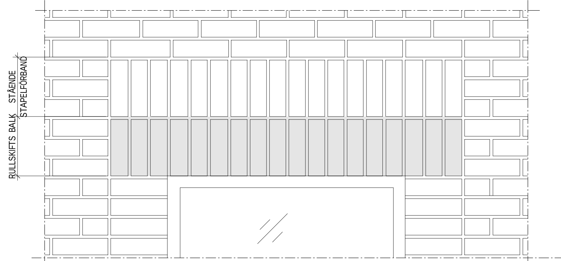
EV2 PRINCIP ELEVATION 1:10 RULLSKIFTS BALK
