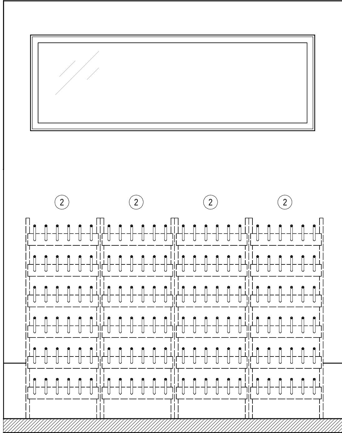
ELEVATION TORKRUM 1002 - A 1 : 20
