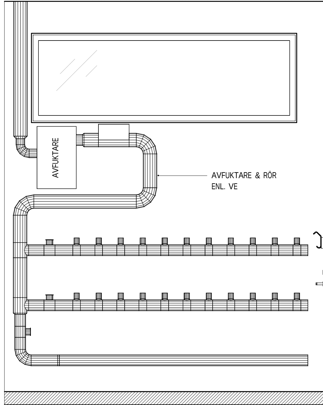
ELEVATION TORKRUM 1002 - C 1 : 20
